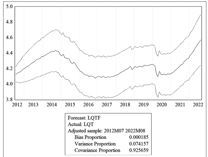
Figure 16: The NARDL forecasting for Qatar stock market (Model with WTI prices)q
