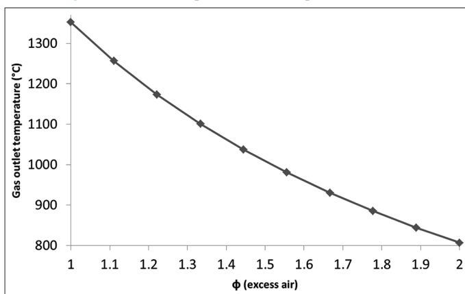
Figure 2: Flame temperature with respect to excess air
