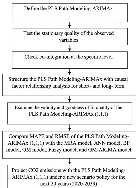
Figure 1: The flowchart of the PLS Path Modeling-ARIMAx. Source: Author’s Estimate (2021)
