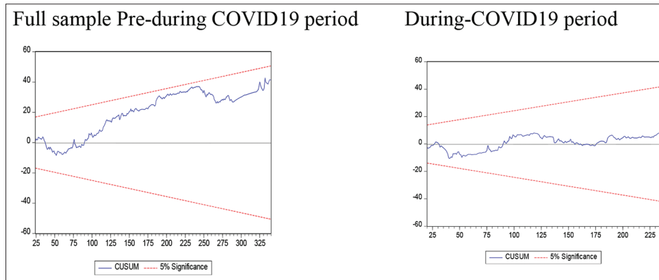
Figure 1: CUSUM test
