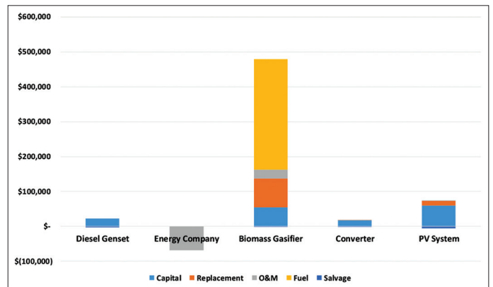
Figure 8: Hybrid system implementation costs for scenario 3 (USD)
